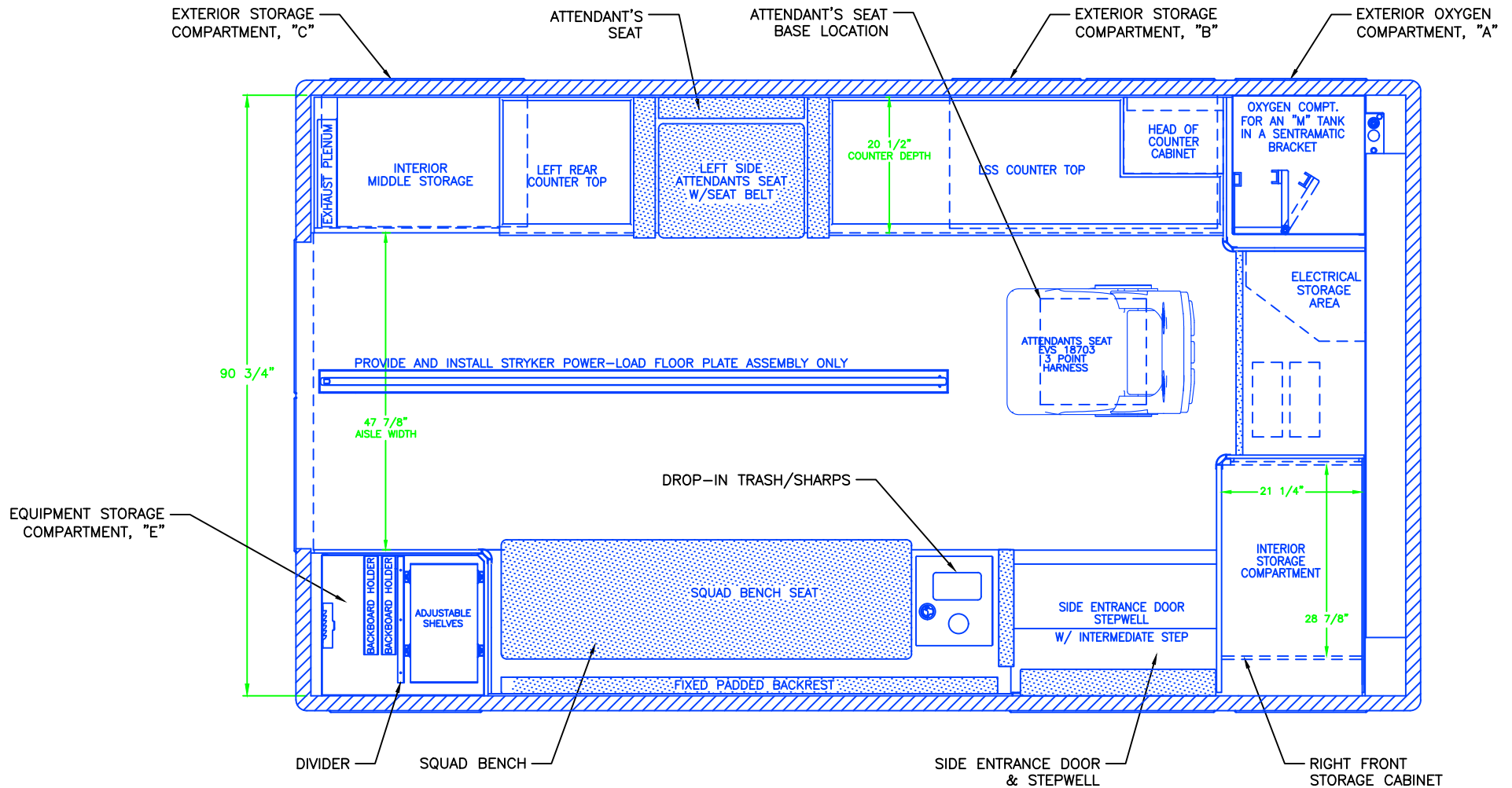
FLOOR PLAN
