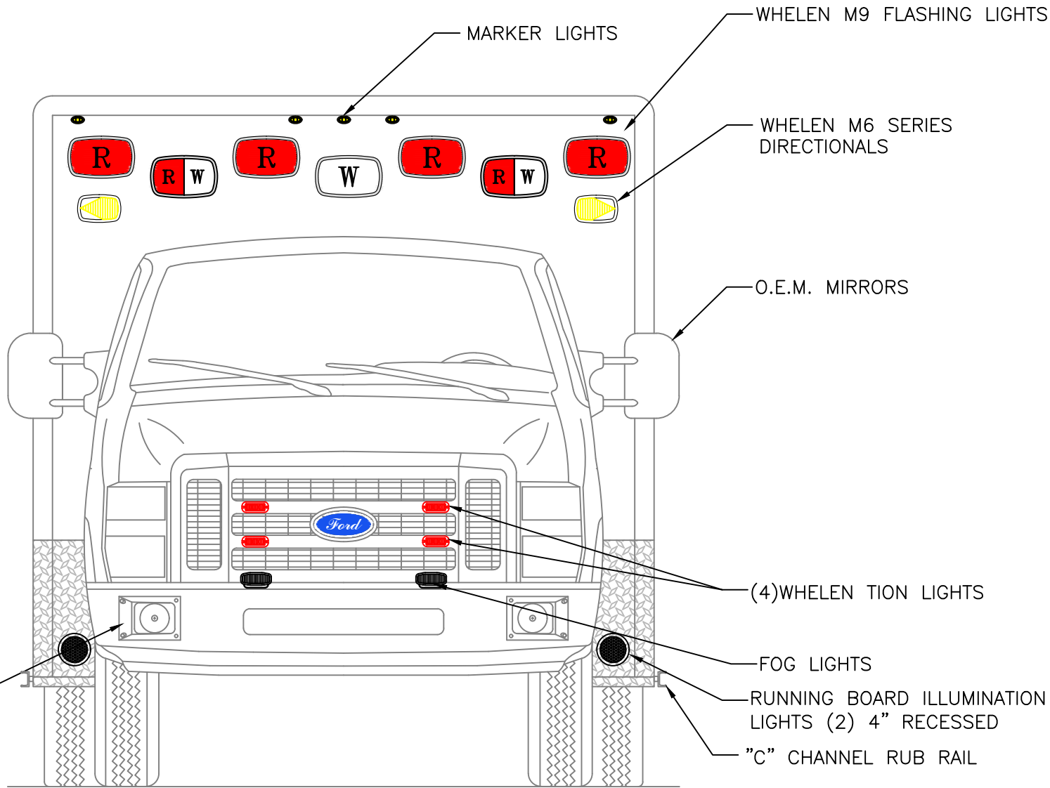
FRONT VIEW
